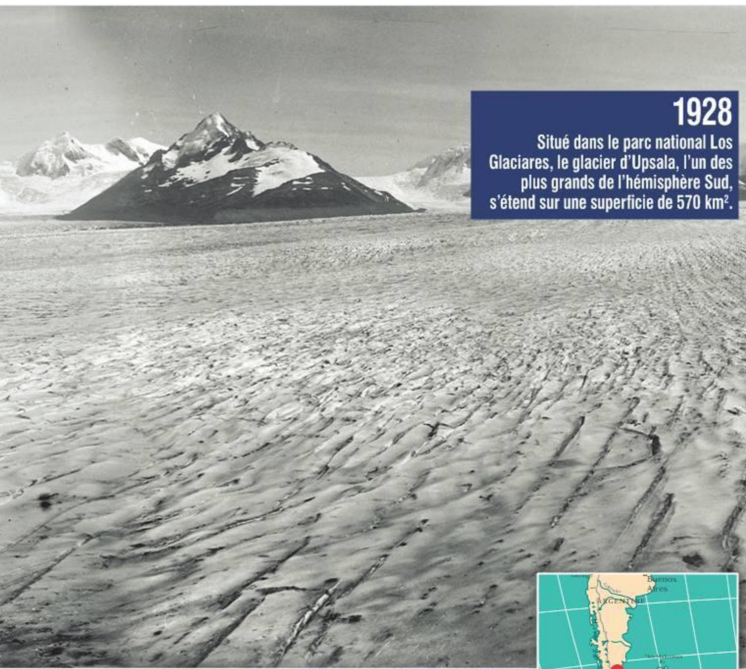
ARGENTINE Glacier Upsala
